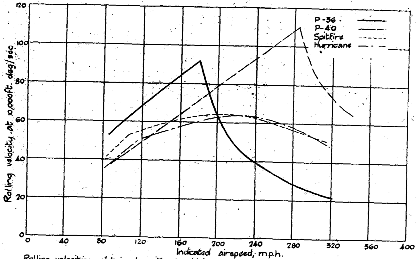
Rolling velocities obtained with a stick force of 30 pounds at 10,000 feet altitude. On straight portions of curves full aileron deflection is reached with less than 30 pounds force.
